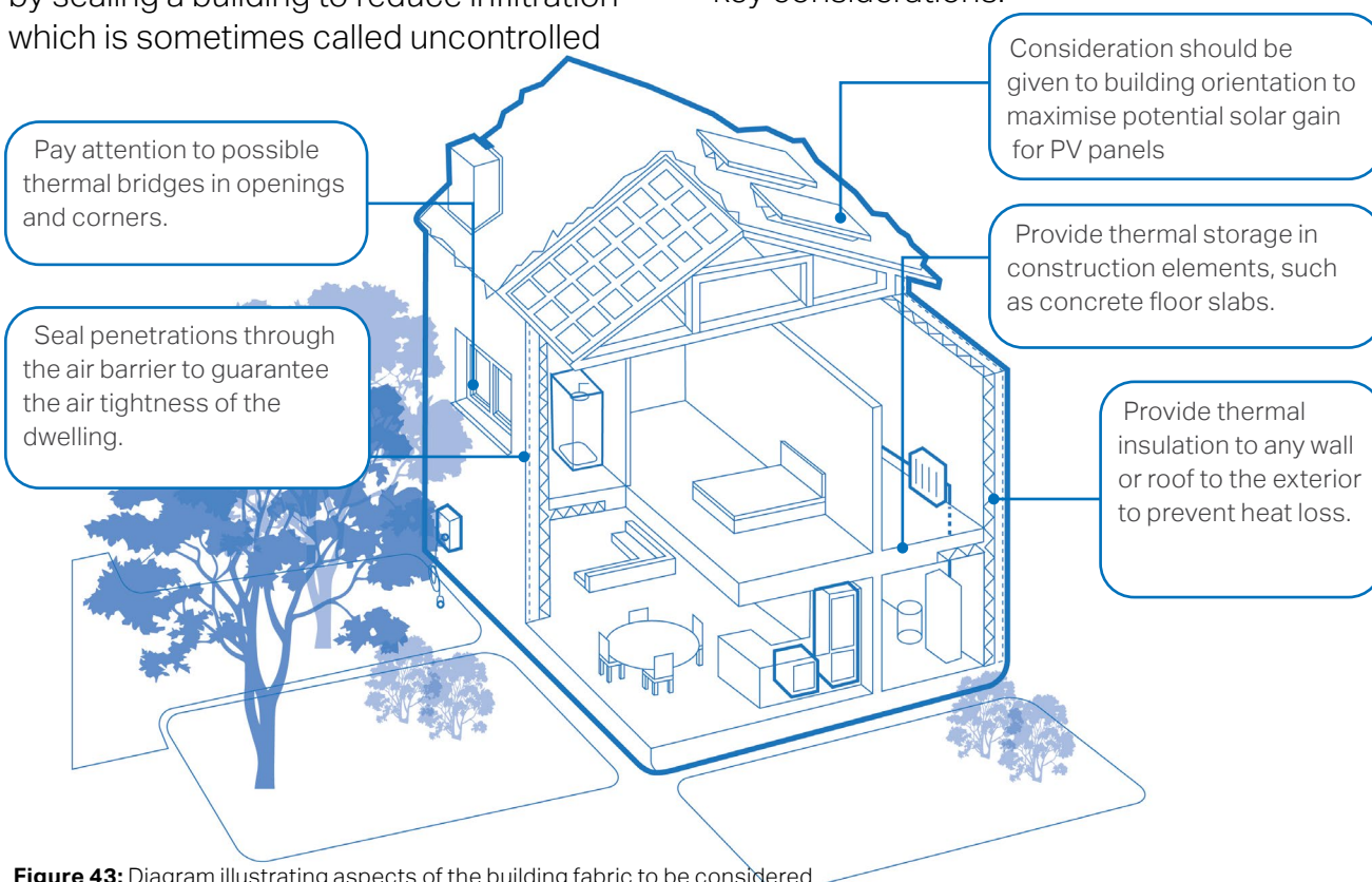
Figure 43: Diagram illustrating aspects of the building fabric to be considered
